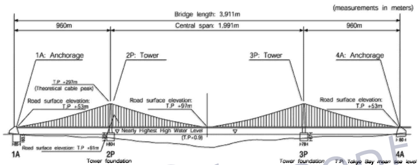
Figure 44: Diagram of the Akashi Kaikyo Bridge showing perfectly parallel suspension towers perpendicular over flat level water.
